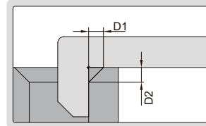
internal chamfer
