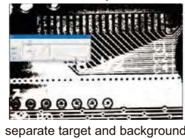
binary
