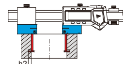
measuring internal groove diameter with spherical measuring face (depth h_2 \geq 7.5\text{mm} )
